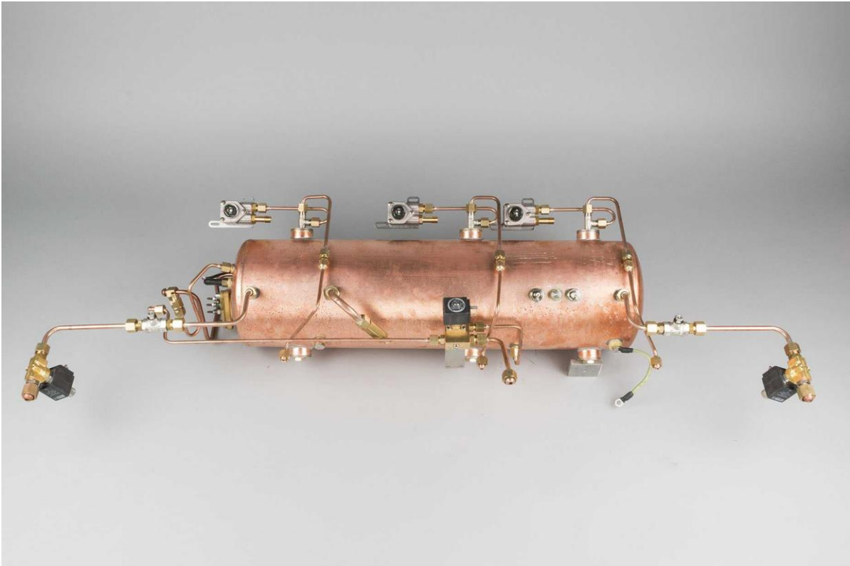
Triplette; steam boiler and ducts, overview
