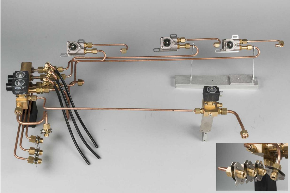
Triplette, pump per group; inlet to manifold to water meter and mix-block, overview
