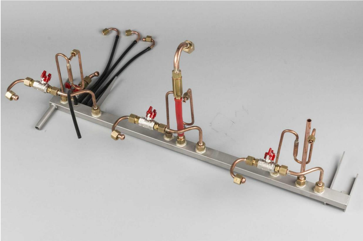
Triplette; discharge, overview
