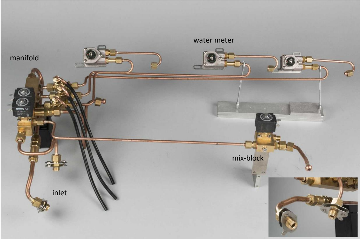
Triplette; inlet to manifold to water meter and mix-block, overview
